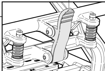
Locking Lever
